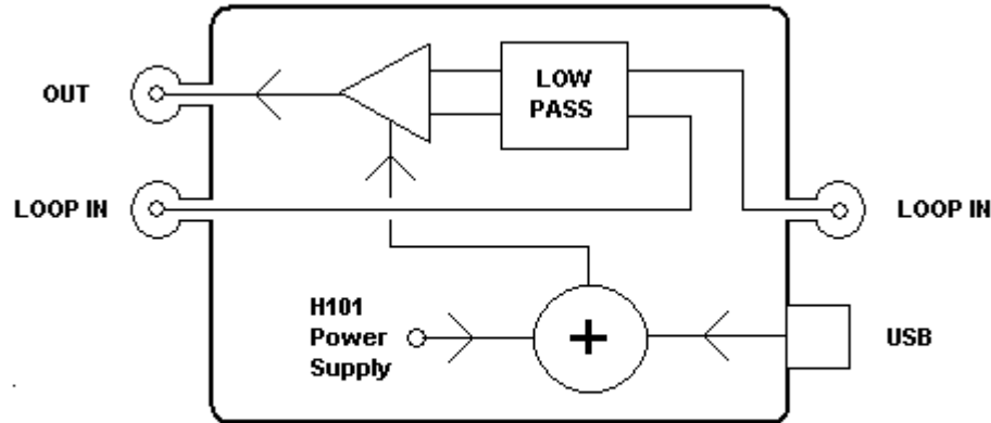
L101 100Khz- 30Mhz ACTIVE LOOP
